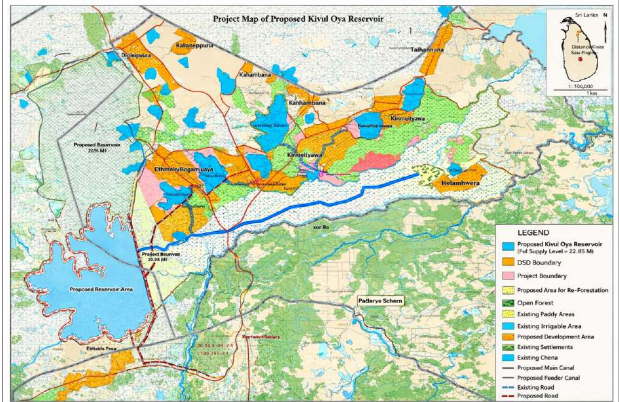
Figure: 2:1 (A) Proposed Project layout map
